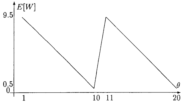
Figure 3: Discontinuous Derivative
